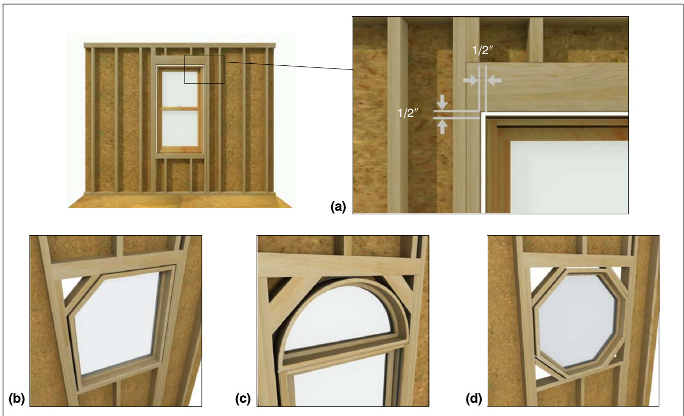
Figure 1: Typical rough and masonry openings.
