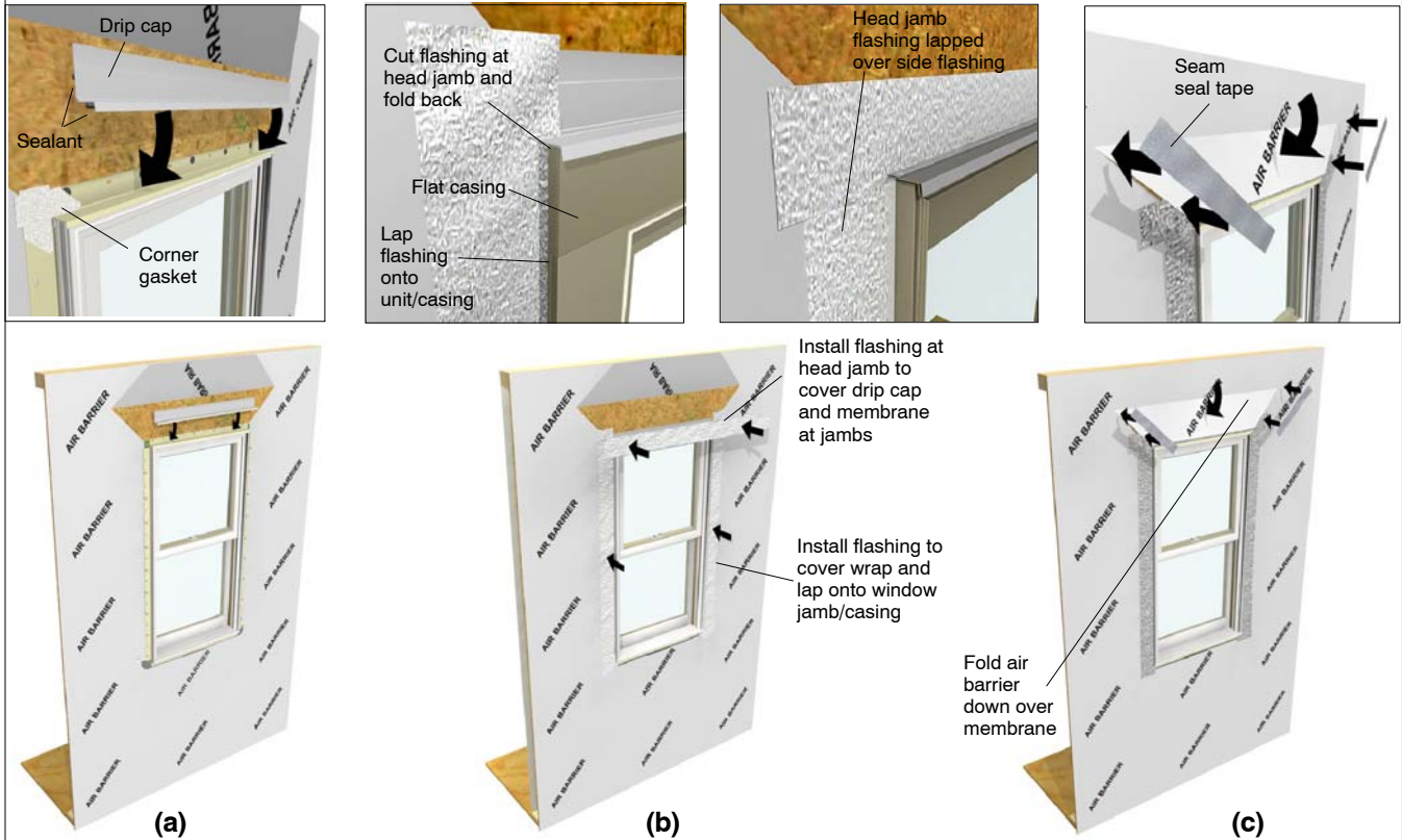
Figure 10: Sealing the Installation in air barrier applications
