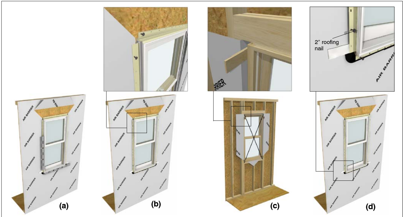
Figure 7: Positioning the window in the opening
