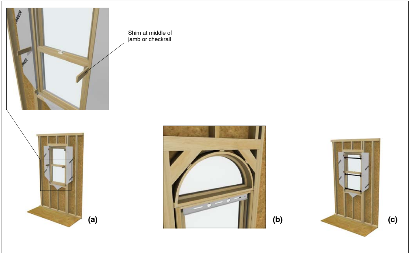
Figure 9: Shimming and squaring the window
