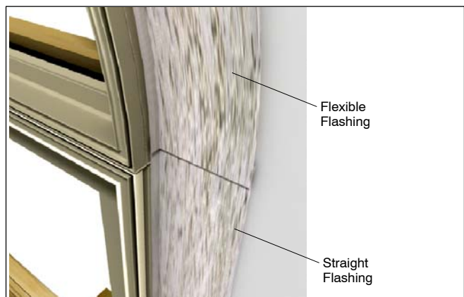
Figure 11: Use flexible flashing for radius head jambs
