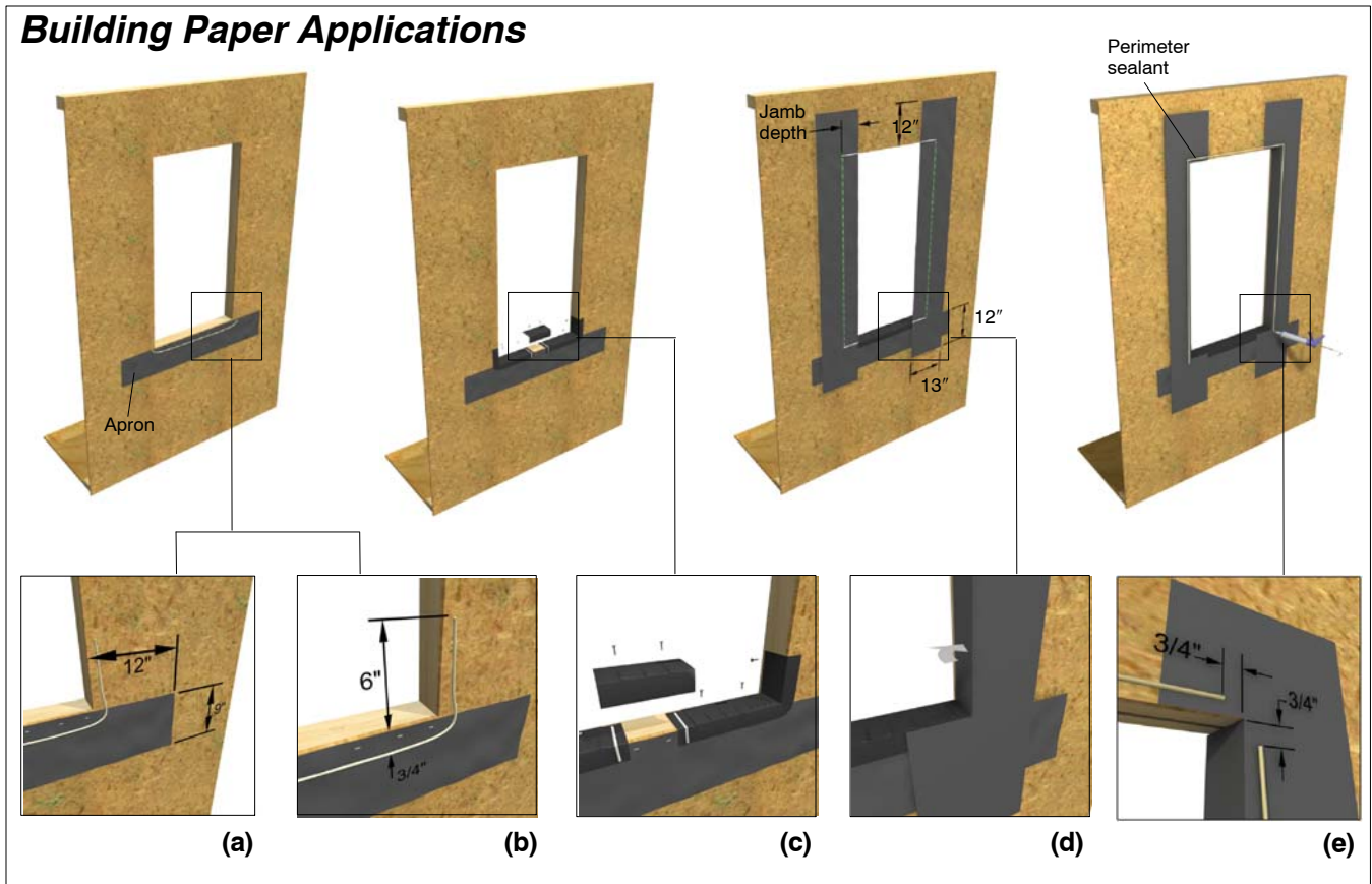
Figure 4: Rough Opening Preparation for construction methods using building paper and rigid sill panning.
