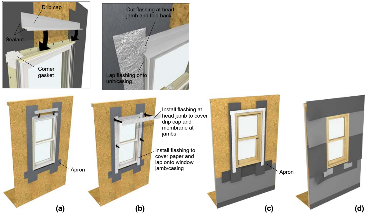
Figure 12: Sealing the Installation in building paper applications
