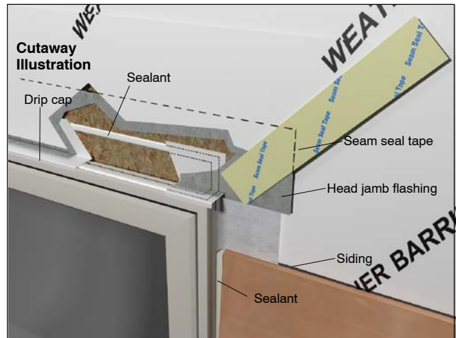
Figure 15: Apply perimeter sealant between window and exterior finish
