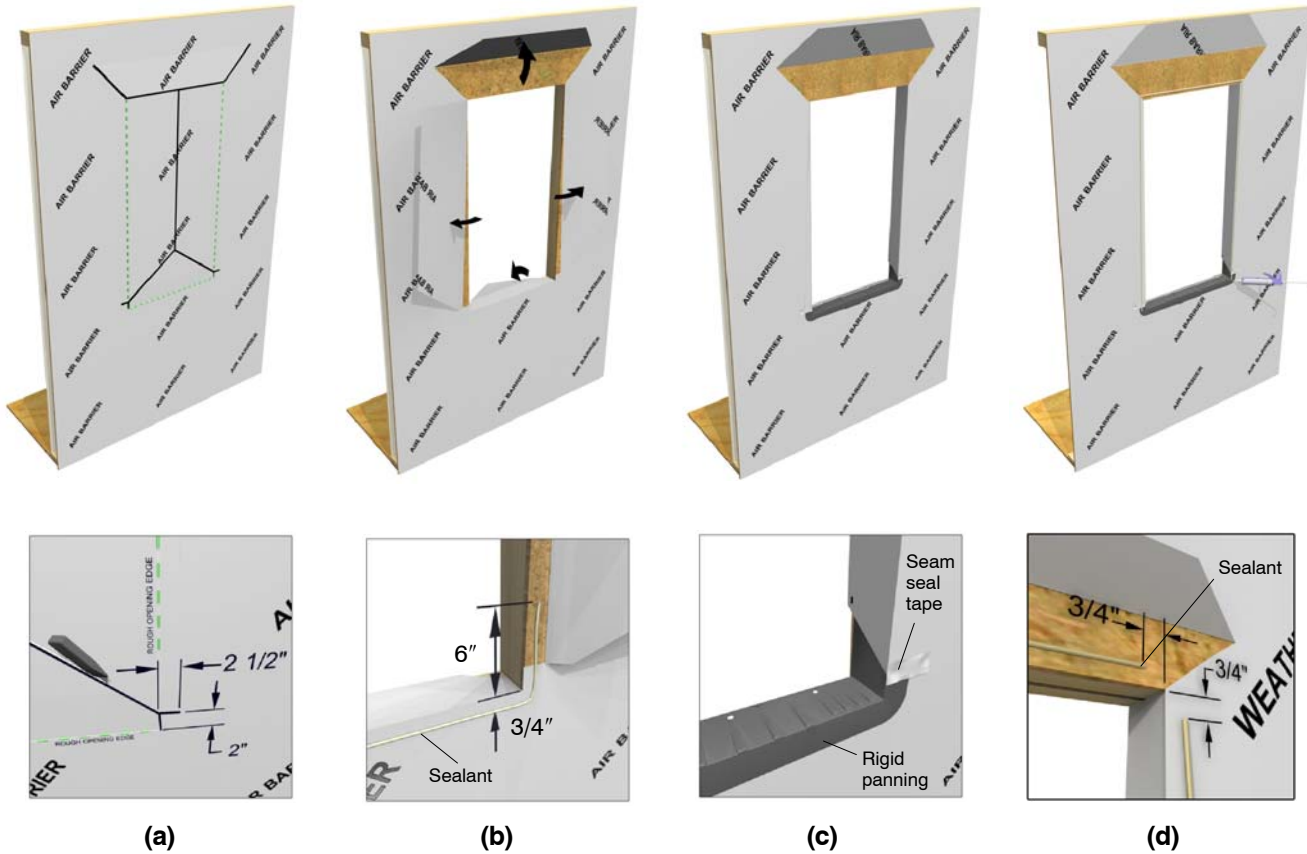
Figure 3: Rough Opening Preparation for construction methods using a continuous air barrier system and rigid sill panning.
